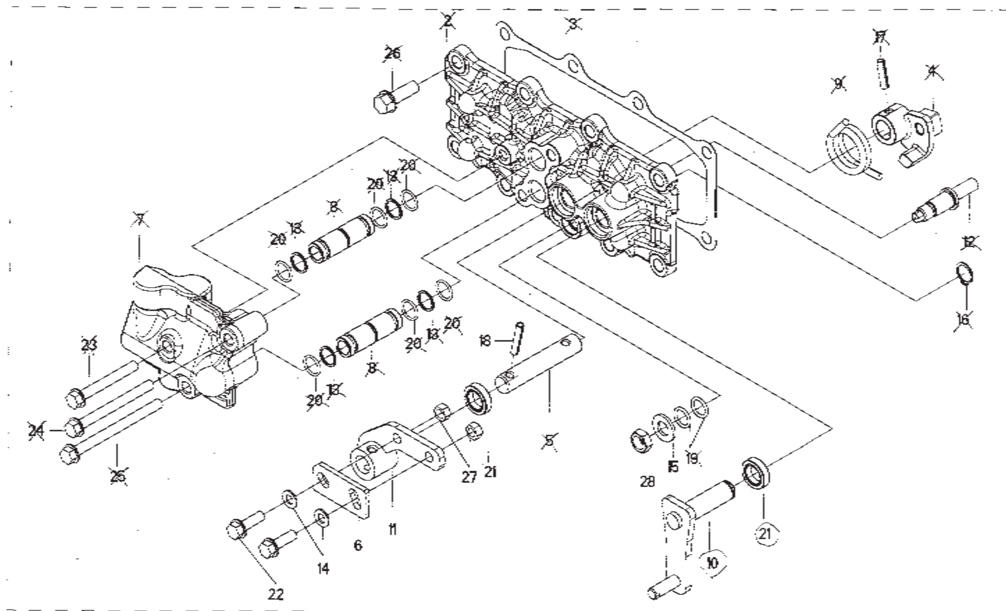
Fig.2 MOTOR COVER ASSY (D87N00-13120)
